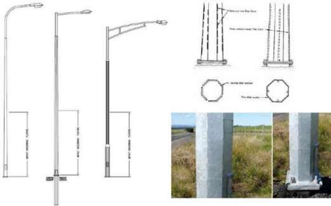
Figura 24: Stâlpi deformabili (Source: Department of infrastructure, Energy and Resources: Road Hazard Management Guide, Tasmania, 2014)
