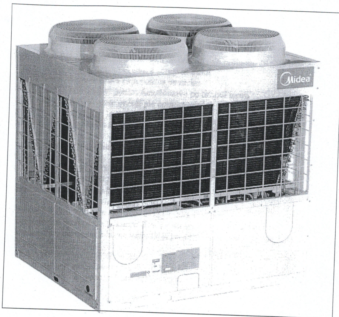
81MD2004---CHILLER HEAT PUMP MIDEA, COMPRESOR ON/OFF, R410A, KIT LOW AMBIENT MGBL-F130W/RN1, 130KW/138KW
